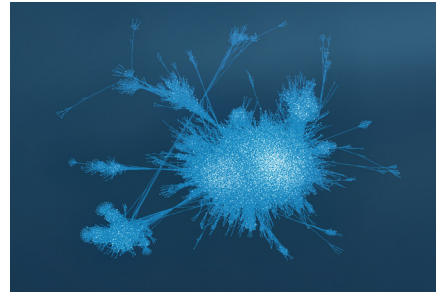
Dependencies
