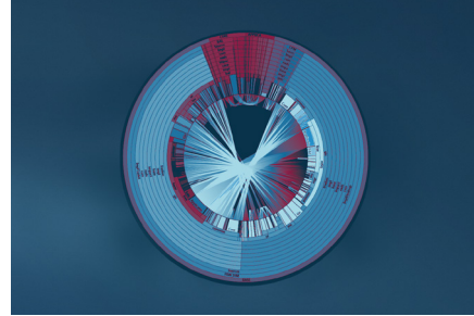
Duplicates
