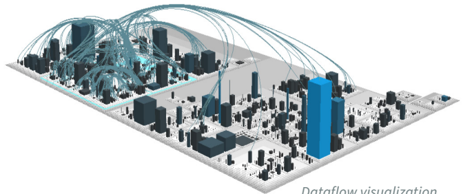
Dataflow visualization
